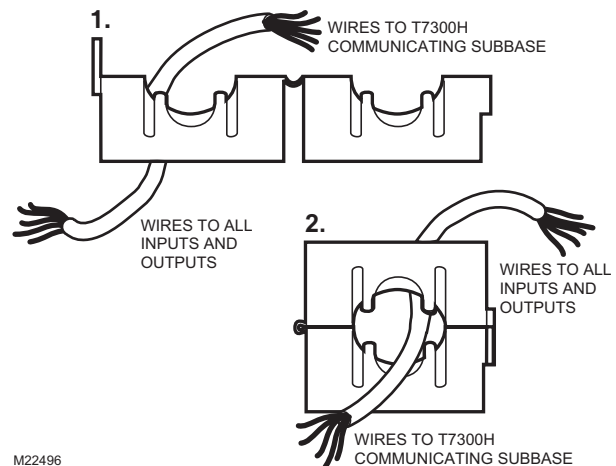
Fig. 8. Ferrite core wires from T7350H to LONWORKS® inputs and outputs.
